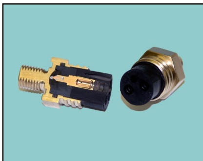
Section of waterblocked Micro WP connector
