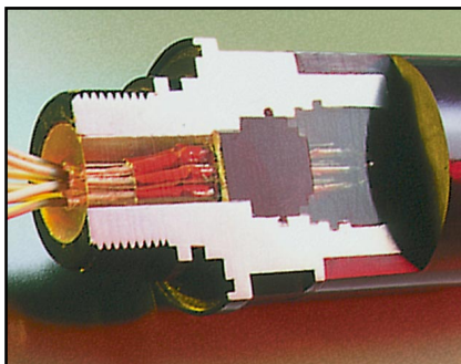
Penetrator construction
