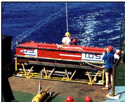
Wet Pluggable Connector application (Courtesy Institute of Oceanographic Sciences)
